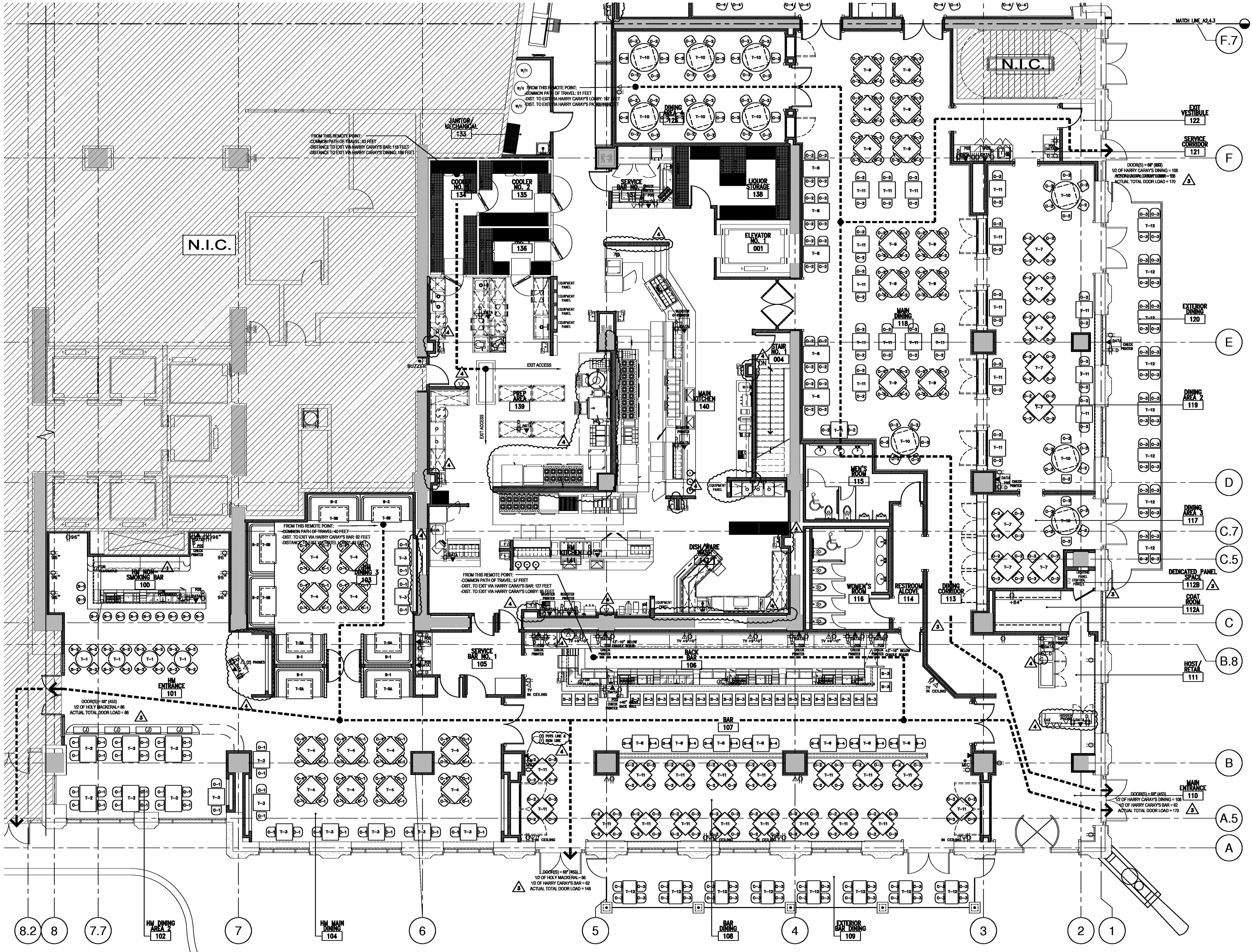
1 SEATING AND EQUIPMENT PLAN (GROUND LEVEL - RESTAURANT AREA) SCALE: 3/16"=1'-0"
