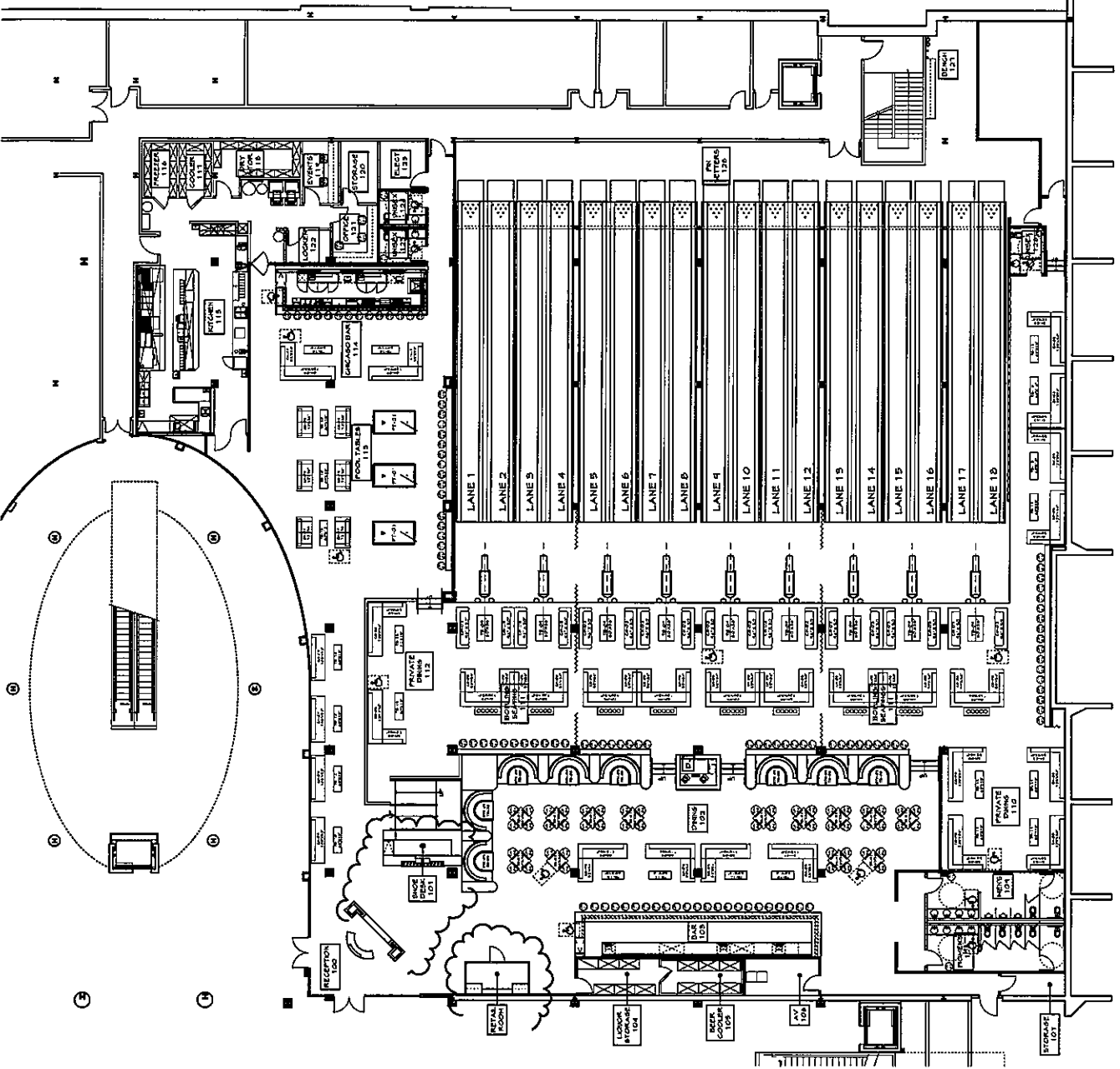
FURNITURE PLAN SCALE: 1/8" = 1'-0"
