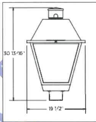
Stresscrete K601D-F2
