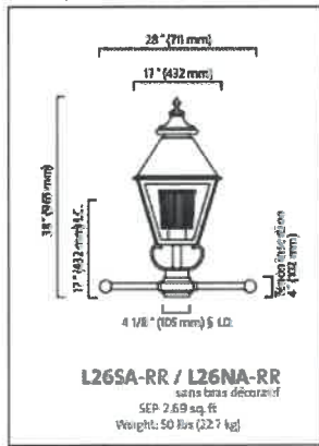
Lumec 100-HPS-L26-C-RR30-240-RSV-5069-BR
