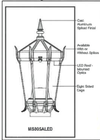
Sternberg MS805BLED
