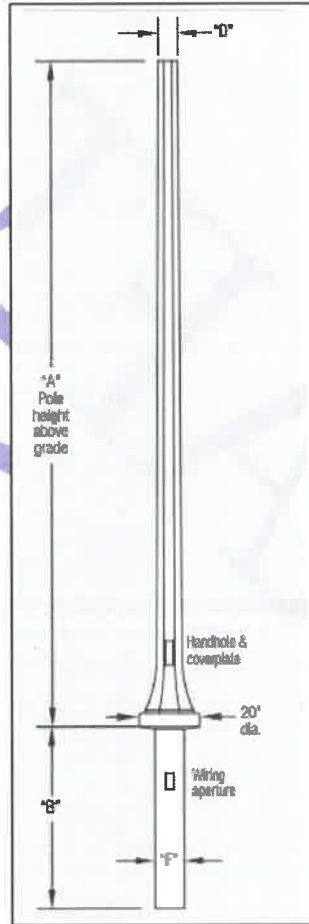
Stresscrete KS15
