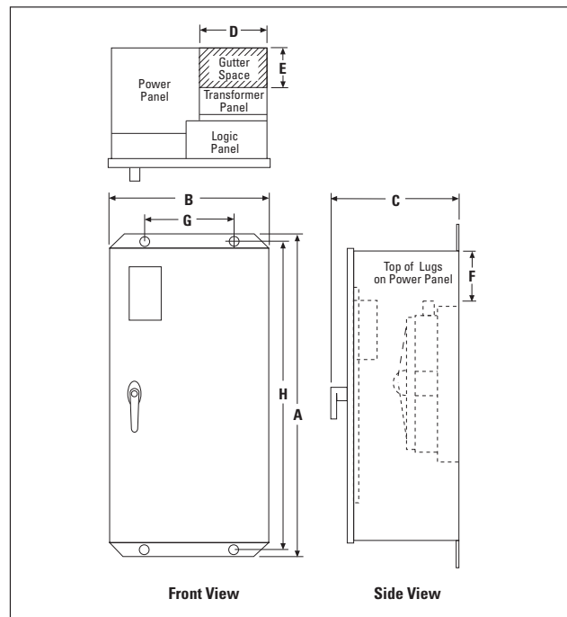
FIGURE 7. DIMENSIONS
