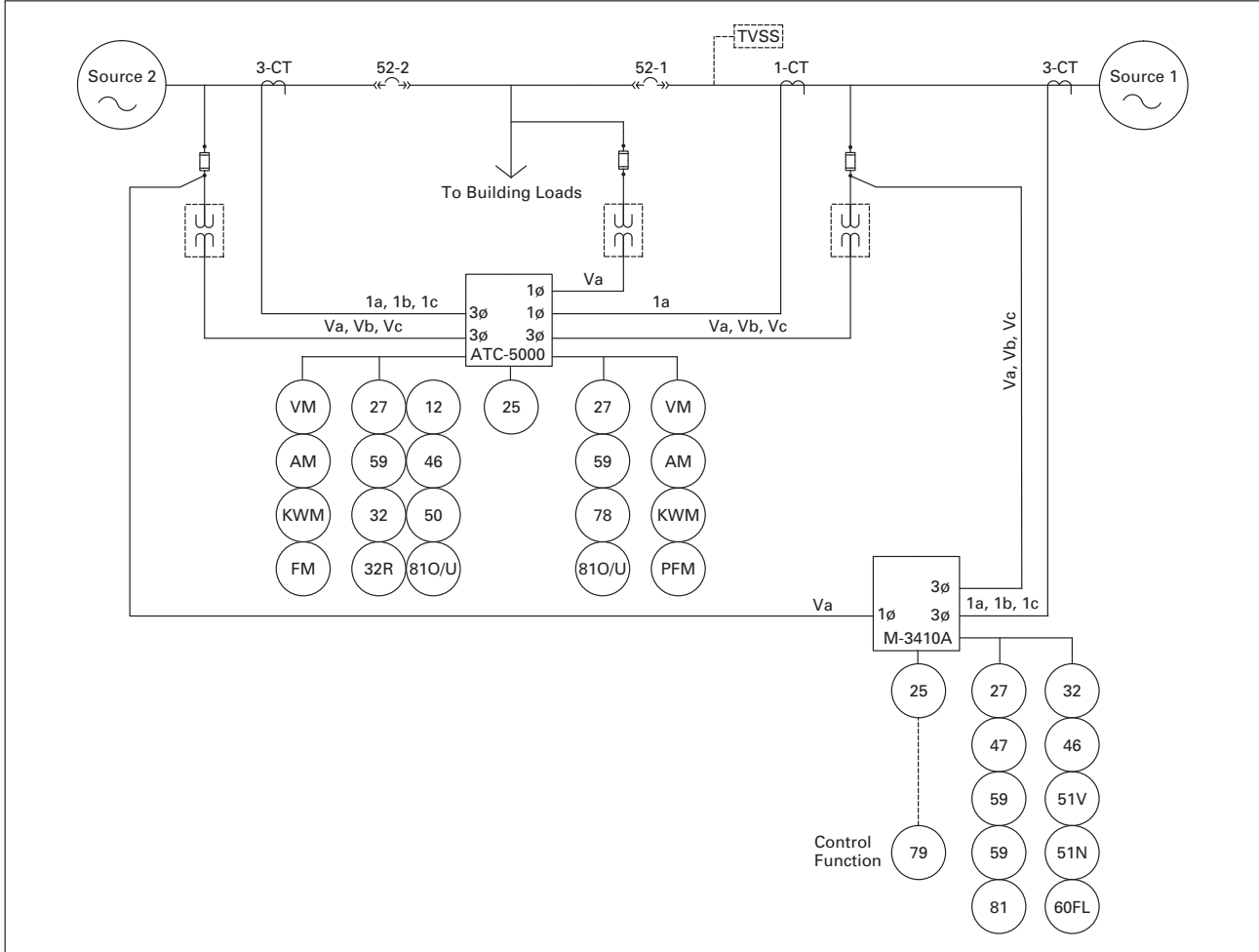
FIGURE 24. TYPICAL SYSTEM DIAGRAM — STANDARD ONE LINE WITH UTILITY GRADE MULTI-FUNCTION RELAYING
