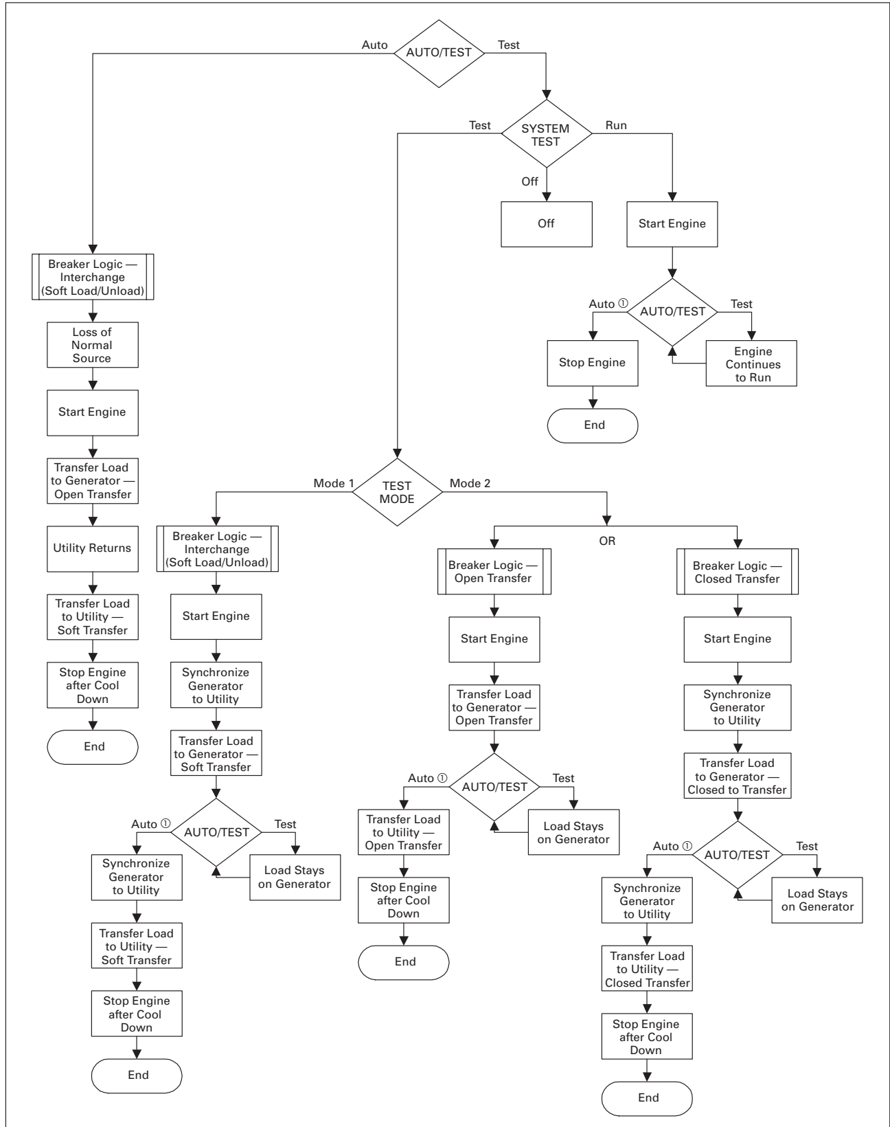
FIGURE 21. SEQUENCE FLOW CHART — SOFT LOAD ATS
