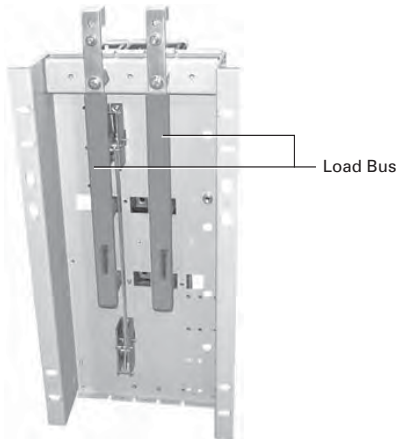
Load Bus
