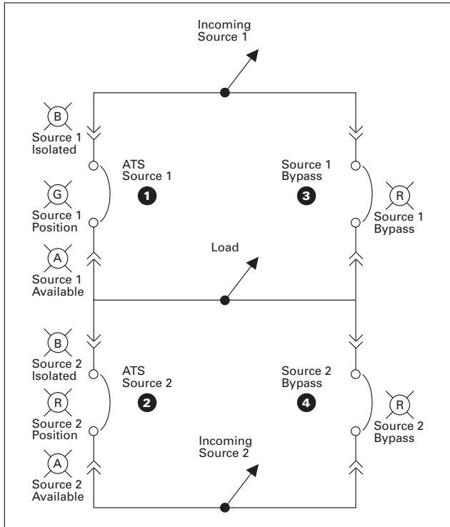
FIGURE 11. TYPICAL BYPASS ISOLATION SWITCH SCHEMATIC
