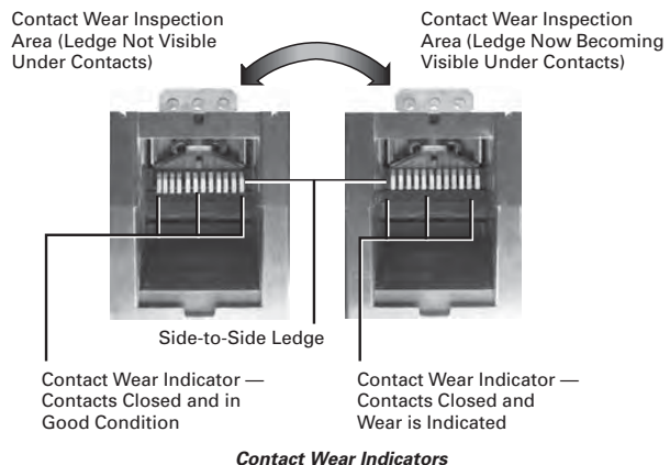
Contact Wear Indicators
