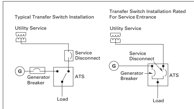
FIGURE 3. SERVICE ENTRANCE RATED TRANSFER SWITCHES
