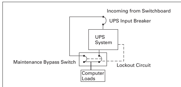
FIGURE 8. SINGLE LINE DIAGRAM OF MAINTENANCE BYPASS SWITCH
