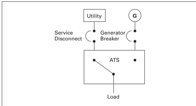
FIGURE 1. STANDARD APPLICATION UTILITY — GENERATOR
