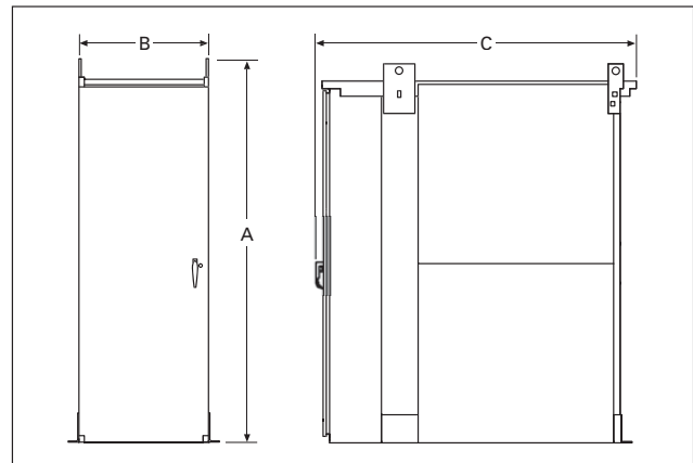
FIGURE 15. 200 – 2000 AMPERE DRAWOUT NEMA 3R
