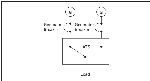
FIGURE 2. STANDARD APPLICATION GENERATOR — GENERATOR
