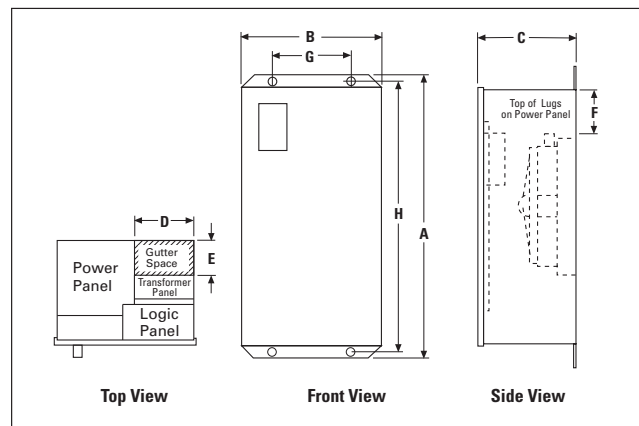
FIGURE 6. DIMENSIONS
