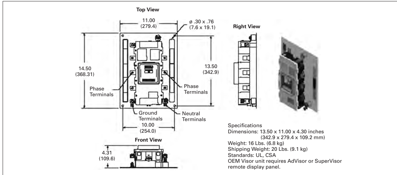
FIGURE 20. VISOR OEM 100, 100 AND 200 KA TECHNICAL DATA
