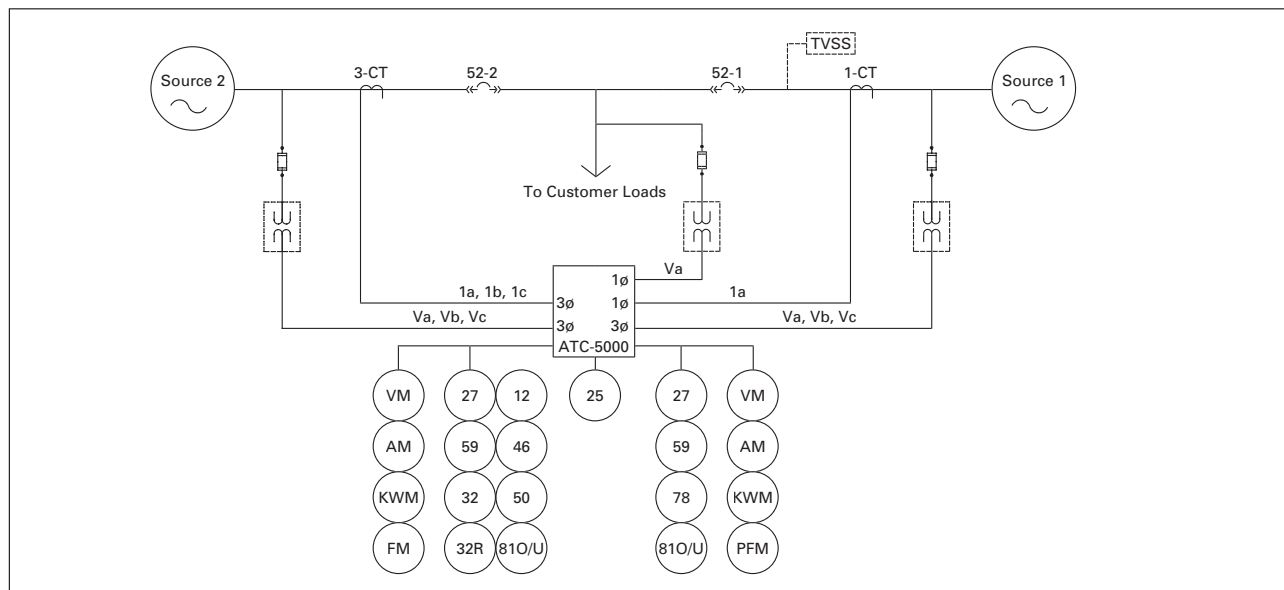
FIGURE 23. Typical System Diagram — Standard One Line
