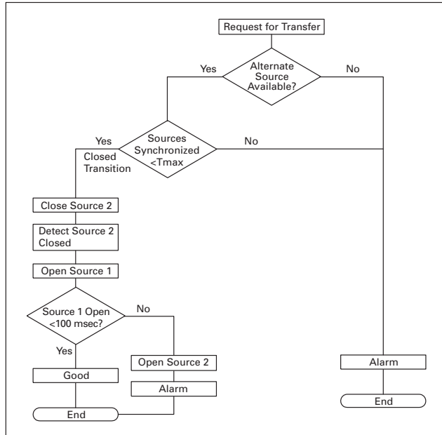
FIGURE 19. FEATURE SET 47D SCHEMATIC
