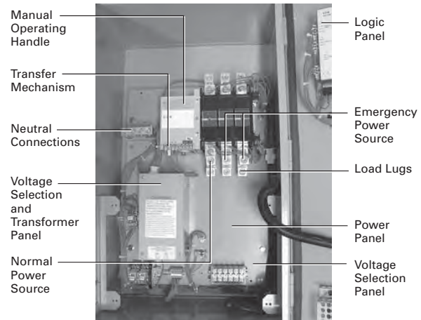
Typical Contactor-Based ATS 100 – 600 Amperes
