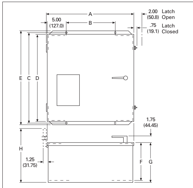
FIGURE 5. DIMENSIONS
