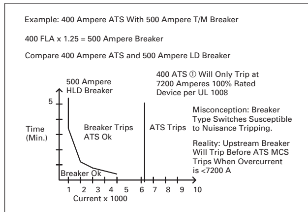
FIGURE 4. BUILT-IN PROTECTION
