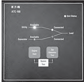
ATC-100 Controller
