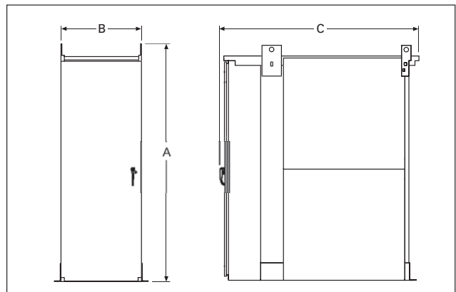
FIGURE 13. 200 – 2000 Ampere Fixed Mount NEMA 3R
