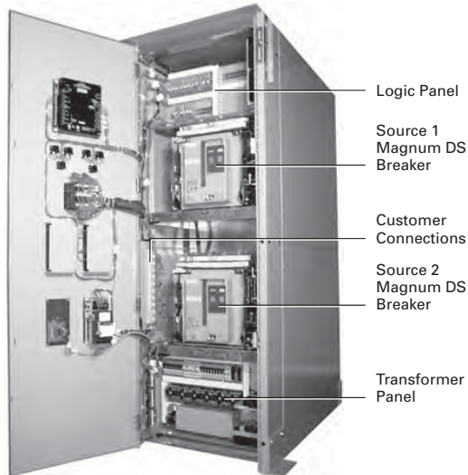
Magnum Soft Load ATS Base Components
