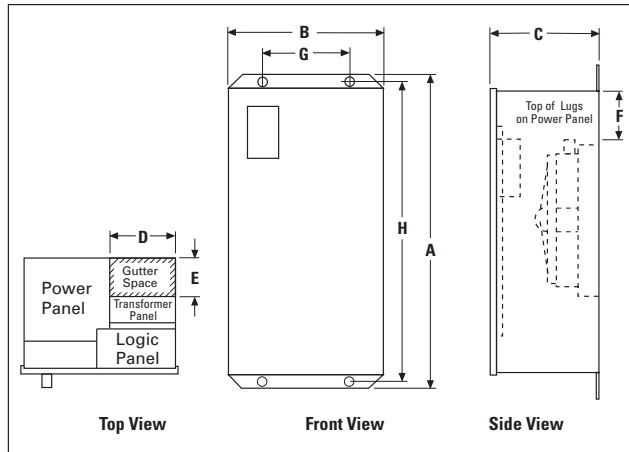
FIGURE 10. DIMENSION VIEWS
