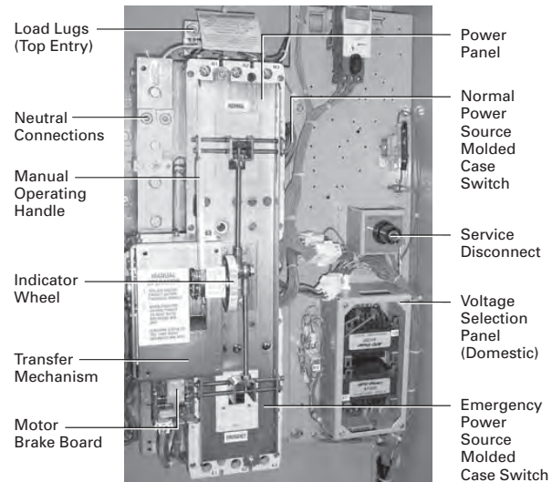
Typical (225 – 1000 Amperes) Vertical Design Transfer Switch Equipment
