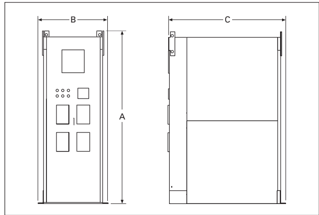
FIGURE 16. 200 – 2000 AMPERE DRAWOUT MOUNT NEMA 1
