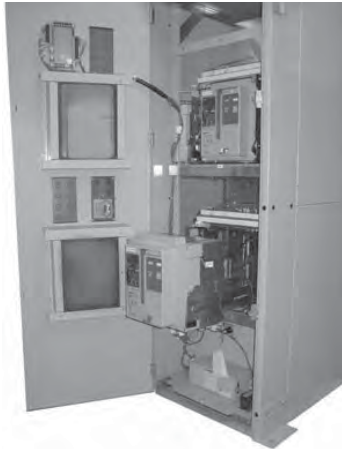
2000 Amperes, 3-Pole NEMA 1 Enclosed Drawout
