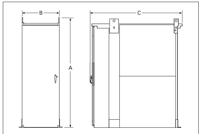
FIGURE 17. 200 – 2000 AMPERE DRAW-OUT MOUNT NEMA 3R
