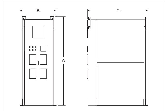
FIGURE 14. 200 – 2000 AMPERE DRAWOUT NEMA 1
