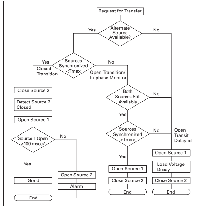
FIGURE 18. FEATURE SET 47C SCHEMATIC
