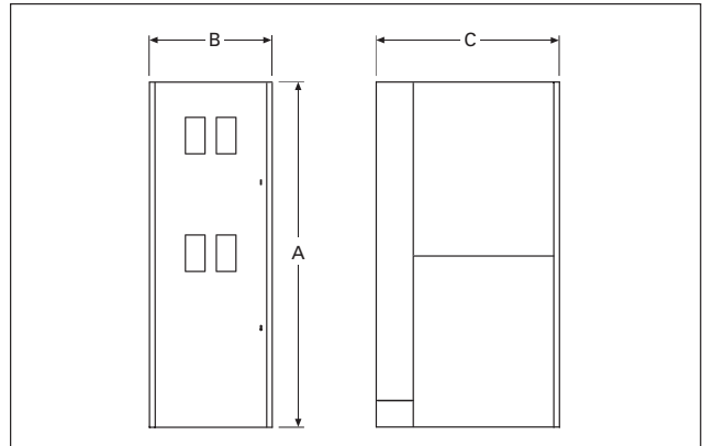
Figure 12. 200 – 2000 Ampere Fixed Mount NEMA 1
