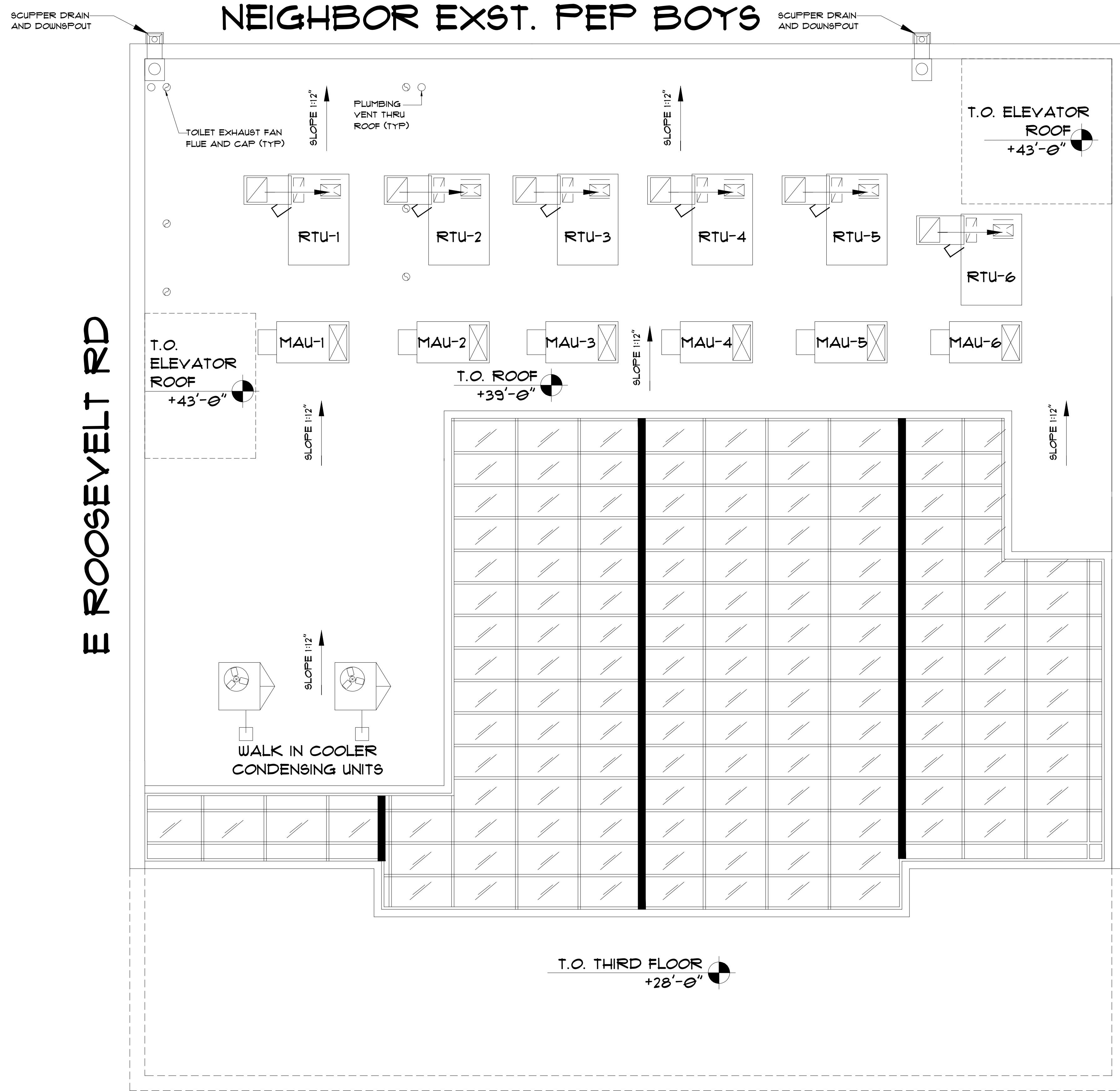
3 PROPOSED ROOF PLAN SCALE: 1/4"=1'-0" NORTH
